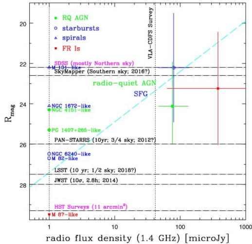
Figure 26 R_{\text{mag}} versus the 1.4 GHz radio flux density for faint radio sources. The diagonal dashed line indicates the maximum value for SFG and the approximate dividing line between radio-loud and radio-quiet AGN, with SFG and radio-quiet AGN expected to populate the top left part of the diagram. The typical R magnitudes of the three classes at S_{1.4} = 1 \mu\text{Jy} are also shown, with SFG split into starbursts and spirals. Finally, the mean radio and R_{\text{mag}} values for sources from the VLA-CDFS sample, with error bars indicating the standard deviation, are also marked. The horizontal dot-dashed lines indicate the approximate point-source limits of planned and existing surveys.
