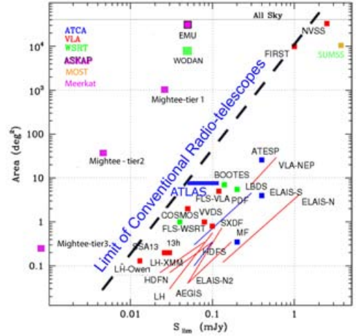
Figure 1 Comparison of existing and planned deep 1.4 GHz radio surveys. The horizontal axis shows the 5\text{-}\sigma sensitivity, and the vertical axis shows the sky coverage. The diagonal dashed line shows the approximate envelope of existing surveys, which is largely determined by the availability of telescope time. For example, to extend NVSS to the sensitivity of EMU would have required over 600 years of (pre-upgrade) VLA time, so in practice this would not have been possible, and this line therefore represents a hard limit to the sensitivity of traditional surveys. The squares in the top-left represent the new radio surveys discussed in this paper. Surveys at other frequencies are not shown in this diagram, as their relative sensitivity depends on the assumed spectral index of the sources, although we do include SUMMS at 843 MHz, without making any correction for spectral index. A similar comparison of low-frequency surveys can be found in Tingay et al. (2012).
