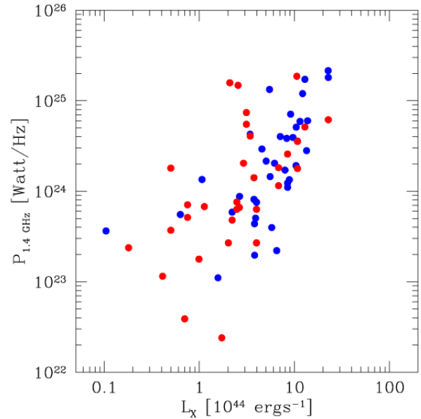
Figure 19 Halo (blue) and relic (red) radio power at 1.4 GHz in units of W/Hz versus cluster X-ray luminosity.
