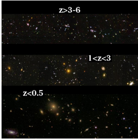
Figure 7 An illustration of the density-dependence of the downsizing of galaxy star formation rates, using optical images from a variety of sources. At the highest redshifts ( z > 3 ), star formation is occurring predominantly in massive galaxies (those that become local massive ellipticals) that live in the most overdense regions (that evolve into today’s massive clusters). At lower redshifts ( 1 < z < 3 ), where EMU/WODAN will be sensitive to the most extreme star forming systems, star formation is dominated by lower mass systems, in less dense environments. By the current epoch, star formation is limited primarily to low-mass galaxies in the outskirts of clusters, and in the lowest-density environments.
