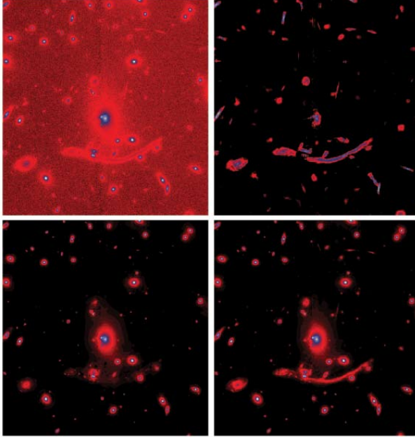
Figure 24 Feature extraction in the HST image of Abell 370 from Starck et al. (2003). The top left panel shows the original HST image, top right shows the co-added image from the ridgelet and the curvelet transforms which extract extended features, bottom left shows the reconstruction from the à trous algorithm which responds to point sources, and bottom right shows the addition of the results of all three transforms.
