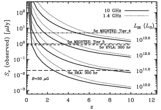
Figure 10 The expected 10 GHz (solid line) and 1.4 GHz (dotted line) flux densities for galaxies of different IR luminosities assuming an intrinsic magnetic field strength of 50 \mu\text{G} . The depths of possible future surveys taken by the VLA, MeerKAT (MIGHTEE), and SKA are shown. Since the non-thermal emission from star-forming galaxies should be suppressed by increased IC scattering of CR electrons off of the CMB, the discrepancy between the point source sensitivity requirements of surveys at 1.4 GHz and 10 GHz falls below a factor of \sim 2 by z \gtrsim 4 .
