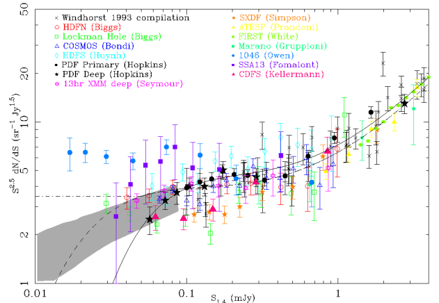
Figure 3 The Euclidean normalised differential radio source counts at 1.4 \text{ GHz} , based on and updated from the distribution shown in Hopkins et al. (2003). The solid curve is the polynomial fit from Hopkins et al. (2003), and the dashed curve is an updated polynomial fit. The horizontal dot-dashed line represents a non-evolving population in a Euclidean universe. The shaded region shows the prediction based on fluctuations due to weak confusing sources (a “P(D) analysis”) from Condon (1974) and Mitchell & Condon (1985).
