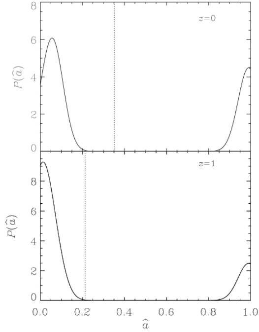
Figure 15 Inferred spin distributions for SMBHs at z = 0 and z = 1 , from Martínez-Sansigre & Rawlings (2011). The vertical dashed lines mark the mean value at each redshift. (Bottom) The spin distribution at z = 1 is dominated by the low-spin population, with a minor component of high-spin SMBHs. (Top) At z = 0 a larger fraction of SMBHs possess a high spin, so that the mean spin is higher.
