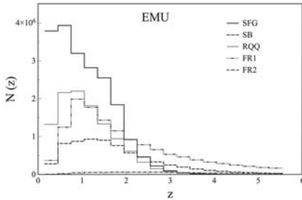
Figure 4 Expected redshift distribution of sources with S_{1.4} > 10 \mu\text{Jy}/\text{beam} , based on the SKADS simulations (Wilman et al. 2008, 2010). The five lines show the distributions for star-forming galaxies (SFG), starburst galaxies (SB), radio-quiet quasars (RQQ), and radio-loud galaxies of Fanaroff-Riley types I and II (FRI & FR2; Fanaroff & Riley 1974). The vertical scale shows the total number of sources expected to be detected.
