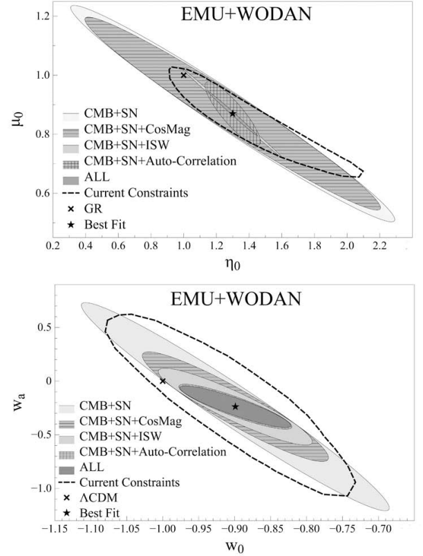
Figure 21 Predicted constraints on parameters using EMU+WODAN. The outer dotted ellipse shows the current constraints, and the innermost grey ellipse shows the constraints available using EMU+WODAN with the three probes described. Bottom panel: dark energy parameters, showing current and predicted 68%CL constraints. Top panel: modified gravity parameter constraints.
