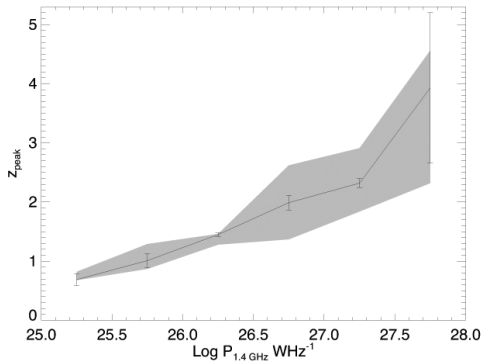
Figure 14 The dependence of the redshift of the peak in space density ( z_{\text{peak}} ) on radio power for the best-fitting steep spectrum grid, showing that the numbers of the most powerful radio sources peak at the highest redshifts (Rigby et al. 2011). The shaded region and error bars give two different determinations of the spread in the measurements.
