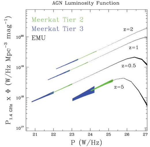
Figure 11 AGN luminosity function at different redshifts expected from the combination of ASKAP and Meerkat deep surveys (based on models described by Prandoni et al. (2007)).
