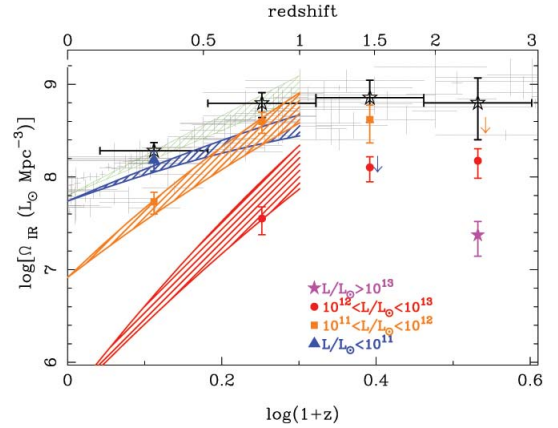
Figure 8 The comoving infrared luminosity density of star forming galaxies as a function of redshift, separated into four infrared luminosity ranges. The shaded regions are from Le Floch et al. (2005) and the bold points are derived from the analysis of faint radio sources in the 13H field (Seymour et al. 2008) where the star-forming radio luminosities have been converted to infrared luminosities using the relation of Bell (2003). The faint, grey points are from the compilation of Hopkins & Beacom (2006) converted to IR luminosity density. The figure shows that ULIRGs make an increasing contribution to the total star formation budget above redshifts of unity.
