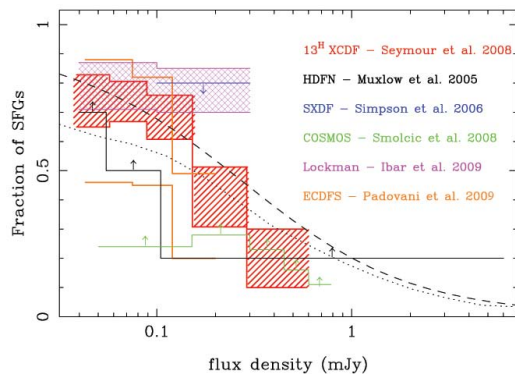
Figure 5 Differential fraction of star-forming galaxies as a function of 1.4 GHz flux density, taken from Norris et al. (2011b). Shaded boxes, and the two lines for Padovani et al., show the range of uncertainty in the survey results. Arrows indicate constraints from other surveys. These results show that the fraction of star-forming galaxies increases rapidly below 1 mJy and, at the 50 \mu\text{Jy} survey limit of EMU/WODAN, about 75% of sources will be star-forming galaxies.
