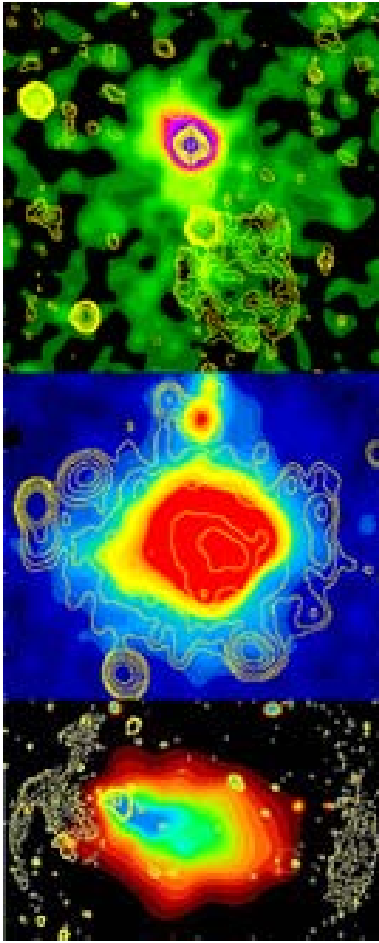
Figure 18 Radio image (contours) overlaid on X-ray images (colour) of three representative clusters: (top) the radio relic in the cluster A1664 (Govoni et al. 2001), (centre) the giant radio halo in A2163 (Ferretti et al. 2001), (bottom) the double relic in A3376 (Bagchi et al. 2006).
