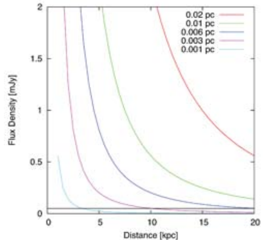
Figure 22 Predicted peak radio flux density of unresolved UCHII and HCHII as a function of distance from the sun. UCHII and HCHII with different diameters are displayed. We assumed a constant electron temperature of 8000 K, a homogenous distribution of material, and high optical depth ( \tau \gg 1.0 ).
