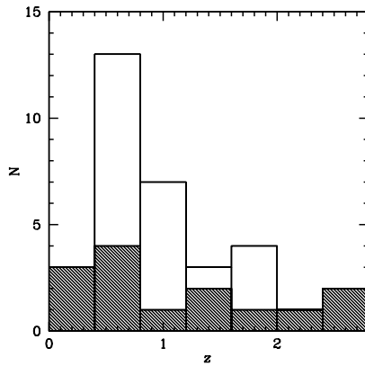
Figure 12 Redshift distribution for radio-faint USS sources in the Lockman Hole, from Afonso et al. (2011). Filled histogram denotes sources with a spectroscopic redshift determination, while the open region refers to photometric redshift estimates. A further 25 USS sources (43% of the full sample) exist but with no redshift estimate, mostly at fainter 3.6 \mu\text{m} fluxes and likely to be found at higher redshifts.
