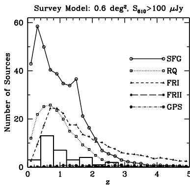
Figure 13 Predictions from the SKADS Simulated Skies models for the redshift distributions of radio source populations, irrespective of their radio spectral indices, for a radio survey reaching a detection sensitivity of 100 \mu\text{Jy} at 610 MHz over 0.6 square degree, similar to the Lockman Hole radio survey considered in Afonso et al. (2011). The observed redshift distribution for USS sources in that work is also displayed.
