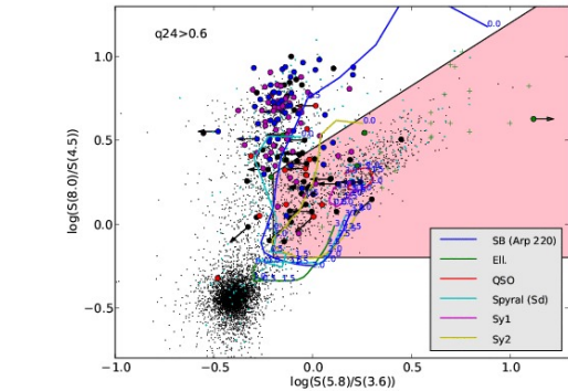
Figure 6 IRAC colour-colour plot of the FLS radio sources with q_{24} = \log(S_{24\mu}/S_{1.4\text{GHz}}) > 0.6 (filled symbols), from Prandoni et al. (2009). Colours refer to optical spectral classification: star-forming galaxies (blue); narrow/broad line AGN (green); early-type galaxies (red); galaxies with narrow emission line, which do not have a secure optical classification (magenta); sources with no optical spectroscopy available (black). Arrows indicate upper/lower limits. The lines indicate the expected IRAC colours as a function of redshift for different source types (see legend). The expected location for AGN is highlighted in pink. For reference we also show IRAC colours of: (a) all FLS IRAC-identified radio sources (no optical identification selection applied, cyan dots); (b) the entire FLS IR-selected star/galaxy population (no radio selection applied, black dots); and (c) a sample of high redshift obscured (type-2) quasars (Martinez-Sansigre et al. 2006), green crosses.
