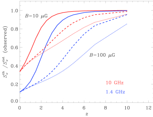
Figure 9 The fraction of radio emission of SFG due to thermal processes as a function of redshift. Galaxy magnetic fields of 10 (solid lines), 50 (dashed lines), and 100 \mu\text{G} (dotted lines) are shown. The radio emission from observations at 10 GHz is dominated by free-free processes beyond a redshift of z \gtrsim 2 even for magnetic field strengths of \sim 100 \mu\text{G} , making it an ideal measure for the current SFR of high- z galaxies (Murphy 2009).
