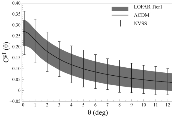
Figure 20 Predicted correlations of the CMB with the LOFAR Tier 1 survey data. As a comparison we also show error bars from current NVSS measurements. Note the improvement we obtain with one of the pathfinders over current constraints on all scales.
