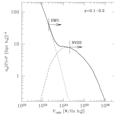
Figure 17 Luminosity functions at 1.4 GHz of giant radio halos in the redshift range 0.1 \leq z \leq 0.2 . The red dashed line marks the contribution from “hadronic” halos in relaxed clusters, while the blue dashed line marks the contribution from halos in merging “turbulent” clusters. The black solid line gives the total luminosity functions (Cassano et al. 2012). The arrows show the EMU and NVSS sensitivities at that redshift.
