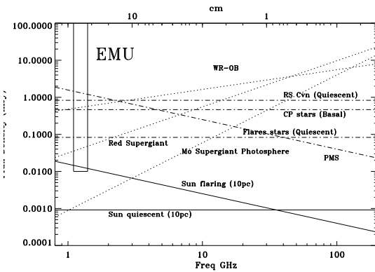
Figure 23 Typical radio spectrum of several classes of radio emitting stars. Fluxes have been derived from the radio luminosity (Seaquist et al. 1993; Guedel 2002; Umana et al. 1998; Triglio et al. 2008; Berger 2006) assuming an appropriate distance for each type of radio star (10 pc for flares stars, including late M-L, 100 pc for active binary systems, 1 kpc for supergiants, OB and WR, 500 pc for CP stars). The bandwidth and sensitivity of EMU have been also indicated.
