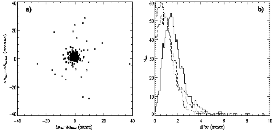
Figure 2.1: a) Differences between the measured positions and those retrieved from SIMBAD for the CIG galaxies. b) Histogram of the difference between the new positions and the SIMBAD positions for the \alpha ( dotted line ), \delta ( dashed line ) coordinates and the total distance ( solid line ) in arcsec. The plotted range is restricted to 10'' for clarity of the plot.
