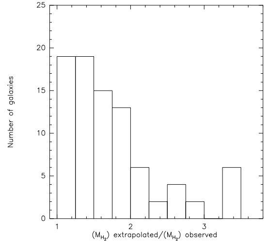
Fig. 2. Distribution of the aperture correction factor for M_{\text{H}_2} .
