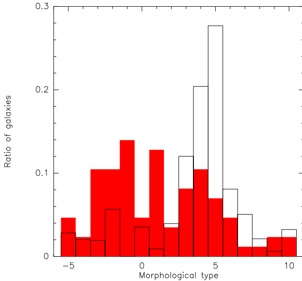
Fig. 1. Morphological types, T(RC3), for the AMIGA isolated (black line) and HCGs (red filled bars) galaxies.
