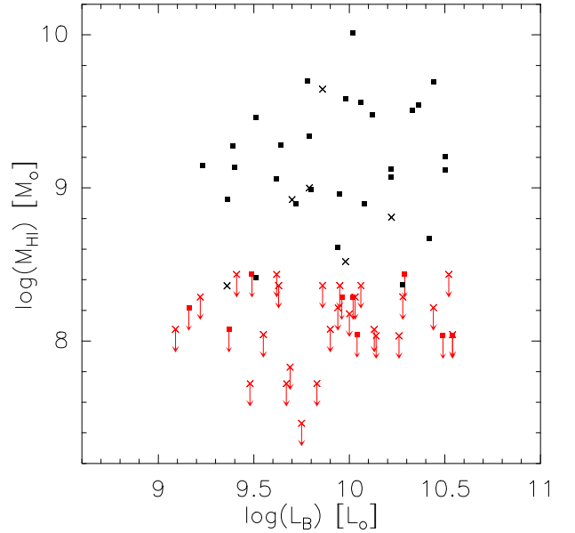
Fig. 5. M_{\text{HI}} vs L_{\text{B}} for late-type ( T \geq 1 , squares) and early-type (crosses) galaxies. Black symbols denote detections and red symbols upper limits.
