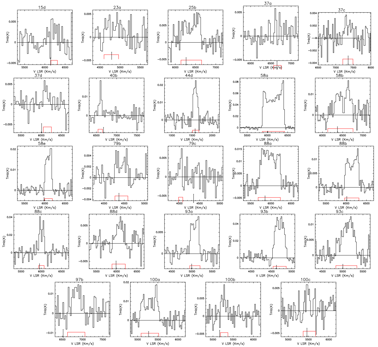
Fig. A.1. CO(1-0) spectra for the detected HCG galaxies. The detection window is shown with a red horizontal line. Main beam temperature ( T_{\text{mb}} , in K) is displayed in the Y axis, and the velocity with respect to LSR in \text{km s}^{-1} is displayed in X axis. Velocity resolution is smoothed to 21 or 27 \text{km s}^{-1} . The optical velocity of the galaxy, converted to the radio definition, is marked with an arrow.
