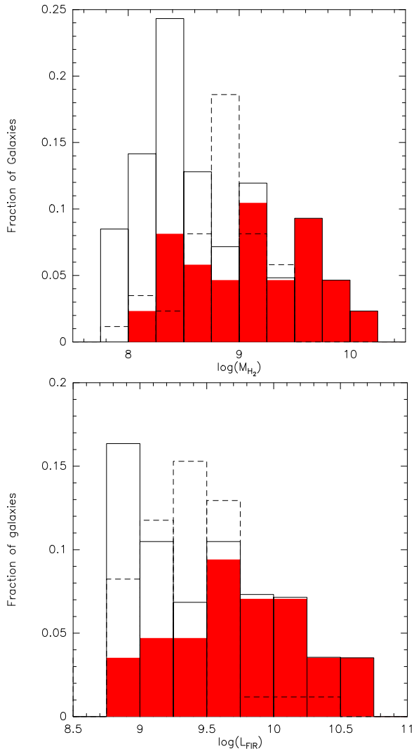
Fig. 3. M_{H_2} and L_{FIR} distribution of the HCG galaxies. The red filled bins show the distribution of the detected galaxies, the dashed line gives the distribution of upper limits and the full line shows the distribution calculated with ASURV.
