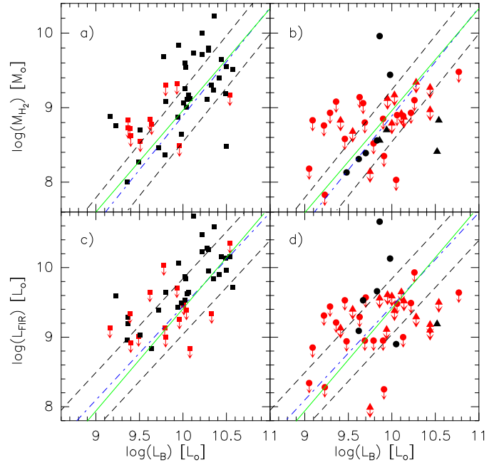
Fig. 4. M_{\text{H}_2} vs L_{\text{B}} for a ) spiral galaxies ( T \geq 1 ) and b ) elliptical (circles) and S0 galaxies (triangles). L_{\text{FIR}} vs L_{\text{B}} for c ) spiral galaxies ( T \geq 1 ) and d ) elliptical (circles) and S0 galaxies (triangles). The full green line corresponds to the bisector fit found for HCG galaxies (fit parameters are given in Table 4), while the blue dashed-dotted line corresponds to the bisector fit found for the AMIGA isolated galaxies. Both fits are done for the entire range of morphological types. The dashed black lines are offset by the standard deviation of the correlation for the isolated galaxies, which is \pm 0.35 for the M_{\text{H}_2} and \pm 0.4 for L_{\text{FIR}} . Black symbols denote detections and red symbols upper limits.
