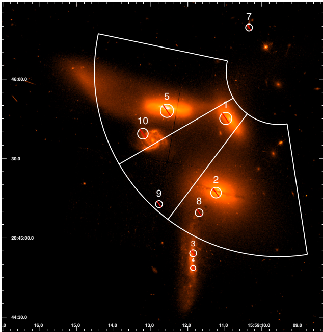
Fig. 5. Regions used to estimate the emission of HCG 79 relative to its members are shown on the HST image (see text). The first wedge subtends an angle from 78 deg to 120 deg, the second one from 120 deg to 143 deg, the third one from 143 deg to 189 deg counter clockwise from N.
