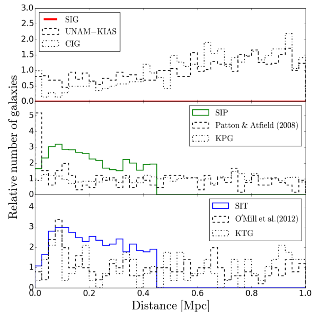
Fig. 5. Normalised distribution of the distance (in Mpc) for neighbours with \Delta v \leq 500 \text{ km s}^{-1} within 1 Mpc around galaxies in the comparison samples. ( upper panel ): The red solid histogram representing neighbours around our isolated galaxies is zero by definition. The black dashed and black dash-dotted histograms correspond to the distributions for neighbours around galaxies in the UNAM-KIAS and the CIG, respectively. ( middle panel ): Distributions for neighbours around galaxies in the KPG (black dash-dotted histogram) and the catalogue of Patton & Atfield (2008) (black dashed histogram). The green solid histogram corresponds to the distribution of the distance for the B galaxies in our isolated pairs. ( lower panel ): Distributions for neighbours around galaxies in the KTG (black dash-dotted histogram) and the catalogue of O’Mill et al. (2012) (black dashed histogram). The blue solid histogram corresponds to the distribution of the distance for the B and C galaxies in our isolated triplets.
