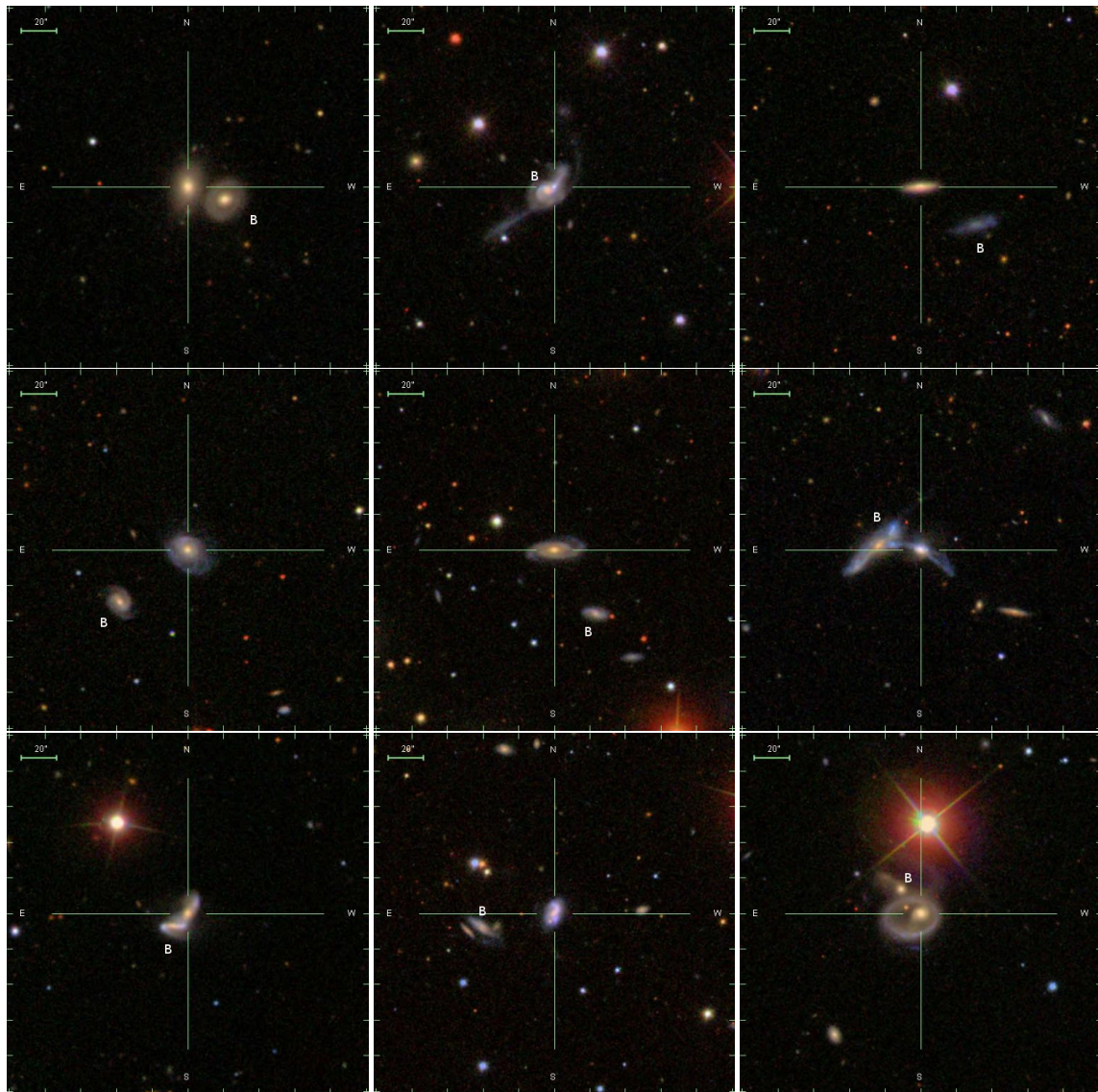
Fig. B.2. SDSS three-colour images (field of view of 3/4 , North is up, East is to the left) of nine isolated pairs in the SDSS-DR10 footprint. The images are centred on the A galaxy. The B galaxy is labelled. From upper left to lower right : SIP 476, 13, 273, 153, 1079, 1123, 515, 1161, and 327.
