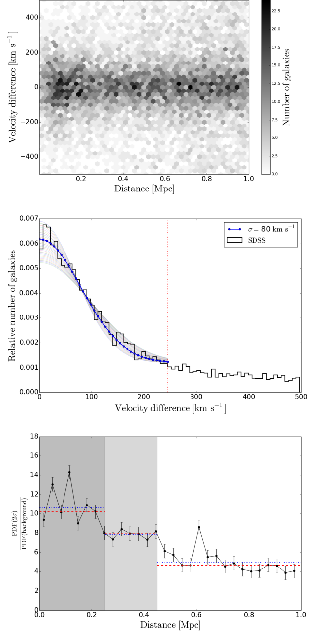
Fig. 1. Selection of physical pairs and triplets. ( upper panel ): 2D distribution of the line-of-sight velocity difference and projected distance for isolated pair and isolated triplet candidates with respect to the brightest A galaxy. Colours correspond to the galaxy counts according to the colour-bar. ( middle panel ): Absolute values of the line-of-sight velocity difference \Delta v = |v_A - v_N| (black histogram), and the corresponding Gaussian distribution fits for \sigma between 70 and 100 \text{ km s}^{-1} (grey curves) with the best fit (blue curve) within the first 250 \text{ km s}^{-1} (red dashed line). The corresponding 2\sigma is shaded. ( lower panel ): Probability Density Function (PDF) for neighbour galaxies within 2\sigma over PDF for the background flat population selected in the interval 300 < \Delta v < 500 \text{ km s}^{-1} , as a function of the distance to the A galaxy. Red dashed and blue dash-dotted lines correspond to the median and mean values in the different distance intervals, respectively. The inner regions up to 250 kpc and 450 kpc are shaded.
