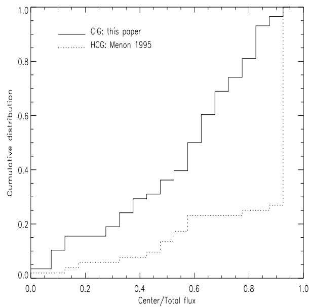
Figure 4.9: Cumulative distribution of the FIRST/NVSS flux ratio for the CIG (solid line) and the center/total flux ratio (dotted line) from Menon (1995). Source: Leon et al. (2008)
