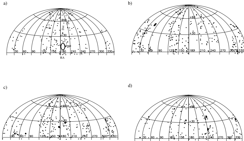
Figure 2.2: Aitoff projection in equatorial coordinates with the location of CIG galaxies divided in radial velocity ranges. The different subplots correspond to the following velocities: a) 0–3000 km s -1 ; b) 3000–6000 km s -1 ; c) 6000–9000 km s -1 and d) 9000–12000 km s -1 . The position of Virgo cluster is indicated with a circle ( \varnothing = 12^\circ ) in panel a), Abell clusters with a richness class of 1 or 2 are also plotted as circles proportional to their radii. Source: Verdes-Montenegro et al. (2005)
