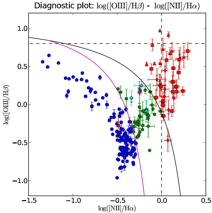
Figure 7.15: Diagnostic plot of \log([\text{OIII}]/\text{H}\beta) and \log([\text{NII}]/\text{H}\alpha) . We plot only galaxies belonging to the SDSS complete subsample ( n = 221 ). AGN galaxies are indicated by red markers, star forming galaxies as blue markers, transition objects as green markers. Non classified galaxies that can be transition objects or star forming galaxies are denoted with cyan markers. CIG 325 can be a transition object or an AGN and is marked with a magenta hexagon. AGN galaxies (red) that are classified as Seyfert 2 are plotted with triangles, the ones that are classified as LINER are plotted with squares and the ones that cannot be classified in any of these subtypes (NLAGN) are plotted as diamonds.
