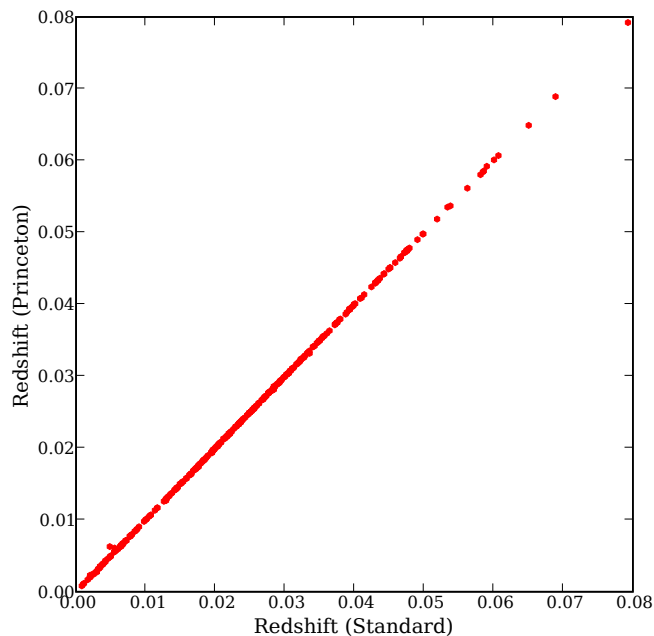
Figure 7.3: Comparison between the redshifts measured with the standard pipeline and the specBS pipeline (Princeton).
