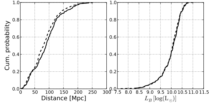
Fig. 2. Cumulative distributions of distance (left) and optical luminosity (right) for the AMIGA (solid line) and SDSS complete samples (dashed line) used in the Kolmogorov-Smirnov two-sample test.
