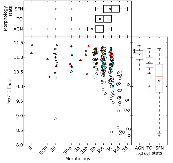
Fig. 8. Properties of the AMIGA isolated galaxies that are in the SDSS complete sample and have available NIR luminosities ( n = 211 ). The main panel shows L_K versus the morphology. The SFN are marked as white round symbols, unclassified galaxies as black + symbols, TOs as cyan squares, and AGN as triangles (red triangles in general and yellow inverted triangles for the Seyfert 1). A small random scatter, like in Fig. 7, was added to the morphology values. The additional panels show the statistics for different types of nuclear activity with respect to the morphology (upper panel) and L_K (right panel). The box marks the lower and upper quartiles, the median is indicated as a red line inside the box, the whiskers extend to the most extreme datapoint within 1.5 \times (x_{75\%} - x_{25\%}) from the median, and the outliers are marked as plus symbols. The mean values are marked using a star symbol. The mean of L_K for Seyfert 1 galaxies is indicated in the right panel with a cross at the left of the AGN box.
