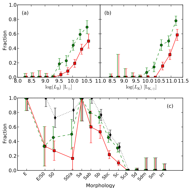
Fig. 9. Relation between the fraction of AGN (red solid line, square symbols) or AGN plus TOs (green dashed line, round symbols) with the optical luminosity (a), NIR luminosity (b), and morphology (c) for the SDSS complete sample. In the morphology panel we also show the fraction (black dotted line, diamond symbols) of AGN plus TOs plus unclassified galaxies (galaxies without detected emission lines that are often referred to in the literature as passive galaxies).
