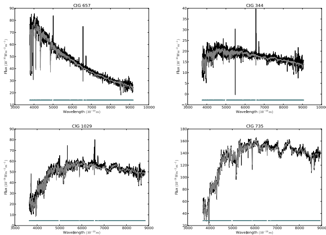
Fig. 4. Example of the fit of the underlying stellar populations performed by Starlight for four AMIGA galaxies with different colours. The original spectrum is shown as a black line, the fitted spectrum as a grey line and the line at the bottom indicates the unmasked region at which the fit was performed. The average ages (log) and metallicities of the depicted galaxies are CIG 657 - 8.8 [a] - 0.005 Z; CIG 344 - 9.4 [a] - 0.015 Z; CIG 1029 - 9.9 [a] - 0.023 Z; CIG 735 - 10.1 [a] - 0.020 Z.
