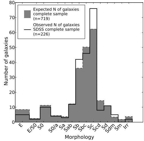
Fig. 3. Binned distributions of morphological types for the observed (open bars) frequencies for the SDSS complete sample and scaled (grey-filled bars) frequencies derived from the CIG complete sample. These frequencies were used to perform a \chi^2 test.
