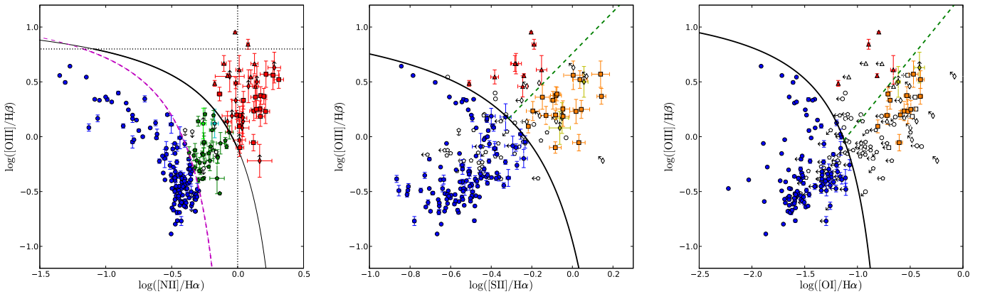
Fig. 5. Emission line diagnostic diagrams. Error bars have been plotted, and an arrow added for upper or lower limits. Left panel: [\text{N II}] diagnostic diagram. The shape of the marker indicates the final classification of nuclear activity: circle - SFN; pentagon - TO; triangle - Sy2; square - LINER, diamond - NLAGN. Filled markers correspond to galaxies classified using this diagnostic diagram, and the colour indicates the derived classification: red - AGN; green - TO; blue - SFN; cyan - TO or SFN; light green - TO or AGN. See Section 3 for a complete description of the classification scheme. Middle panel: [\text{S II}] diagnostic diagram. The AGN-SFN separation curve of Kewley et al. (2001) is shown as a black solid line and the Sy2-LINER separation line of Kewley et al. (2006) as a green dashed line. Symbol shapes are the same as in the [\text{N II}] diagram and the colours indicate the classification obtained with this diagram: red - Sy2; yellow - NLAGN; orange - LINER; and blue - SFN. Right panel: [\text{O I}] diagnostic diagram. Symbol shapes are the same as in the [\text{N II}] diagram. Colours and separation curves are the same as in the [\text{S II}] diagram. Empty symbols correspond to galaxies that cannot be unambiguously classified using this diagram but that were eventually classified using the other diagrams (see text).
