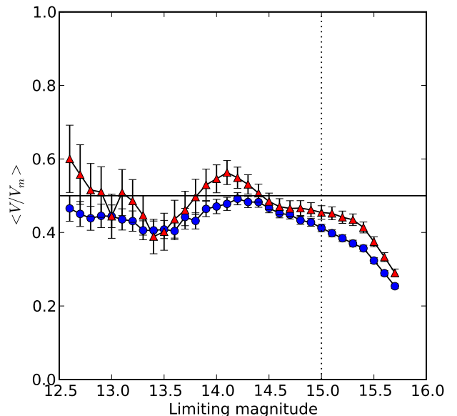
Fig. 1. Result of a \langle V/V_m \rangle completeness test for the CIG SDSS sample ( n = 353 , red triangles) and the CIG full sample ( n = 1050 , blue circles).
