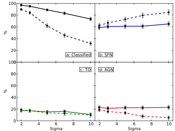
Fig. 6. Fraction of galaxies that are a) classified; b) classified as SFN; c) classified as TO; d) classified as AGN, with respect to the noise level using two different classification methods. The first method is the one presented in this paper that takes into account the information provided by upper limits (solid line, square markers) and the second method is the classical method that takes into account only galaxies with detections of all lines involved in the [N II] diagnostic diagram (dashed line, round markers).
