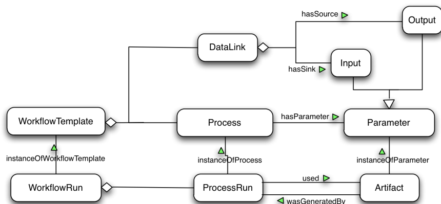
Fig. 2: Resources aggregated within workflow-centric research objects and their relationships. CHECK IF IT IS OK. for instance, abstract workflow does not appear, although it appears on the text, the same on the next figure.
